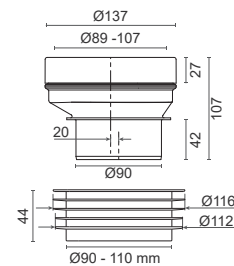
Flexy excêntrico sanita 20 mm Flexy manguito wc 20mm Flexy wc 20mm connector Flexy raccord wc 20mm
