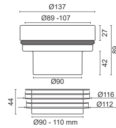
Flexy canhão sanita direito Flexy manguito wc recto Flexy wc straight connector Flexy raccord droit wc
