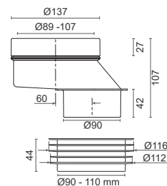
Flexy excêntrico sanita 40 mm Flexy manguito wc 40 mm Flexy wc connector 40 mm Flexy raccord wc 40 mm
